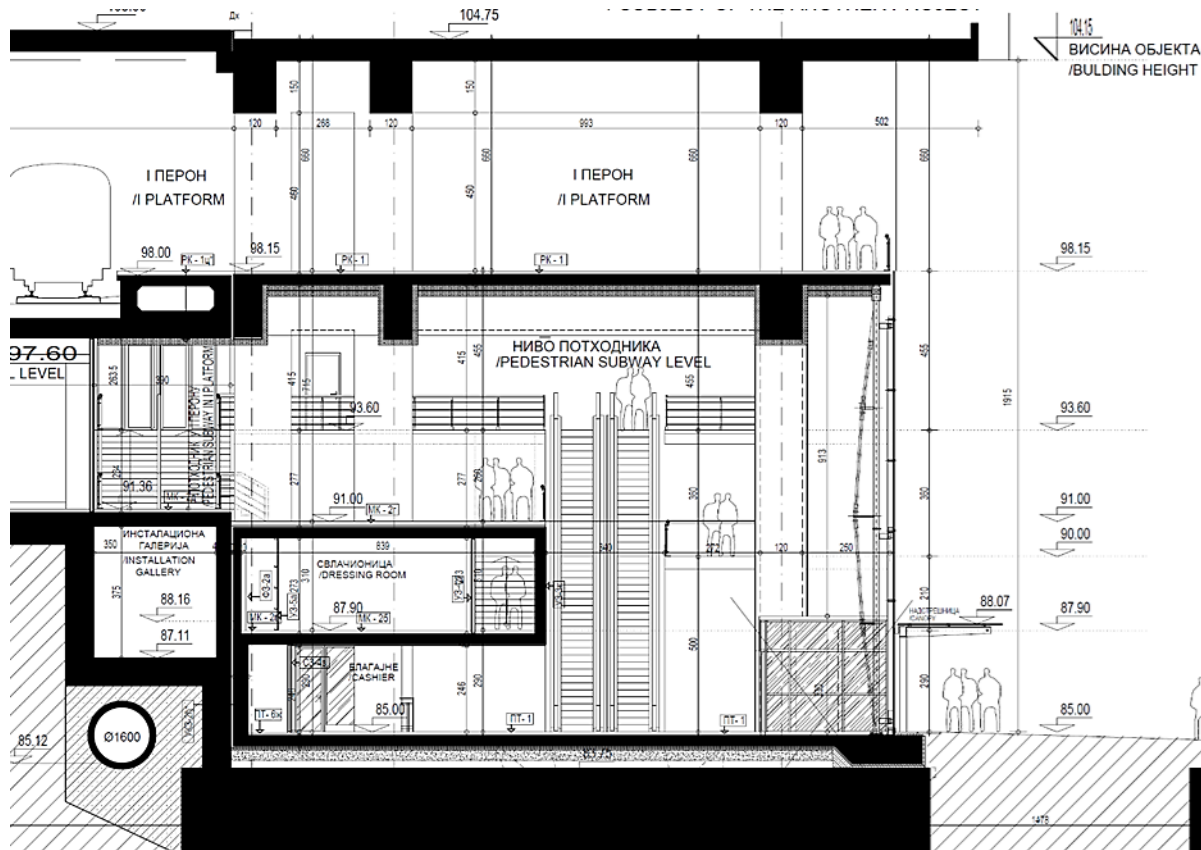
Figure 3. Elevation levels on Belgrade Centre Station below elevation 105,5
