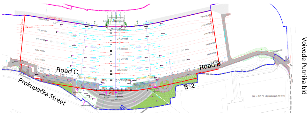
Figure 6: Graphic illustration from Institute of Transportation CIP d.o.o., "Design of Access Roads to the Lower Square, Tracks and Building," Belgrade, 2023.
